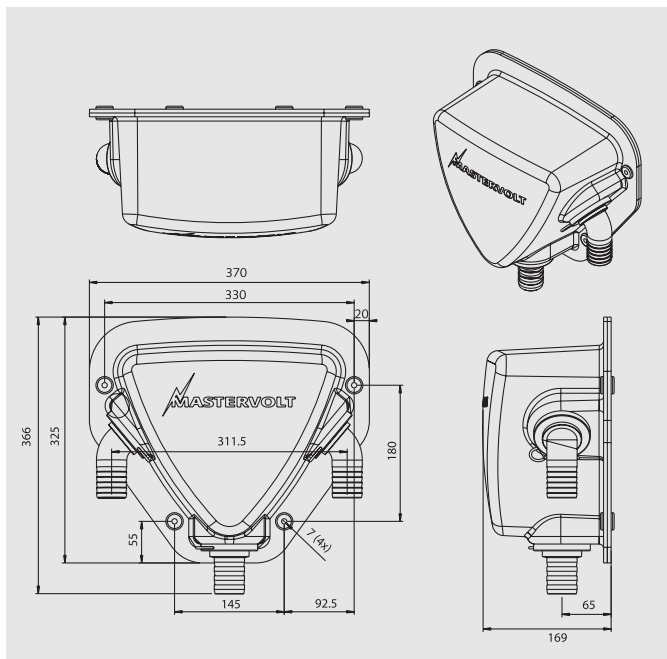
Dimensions in mm of the Delta gas/water separator.
