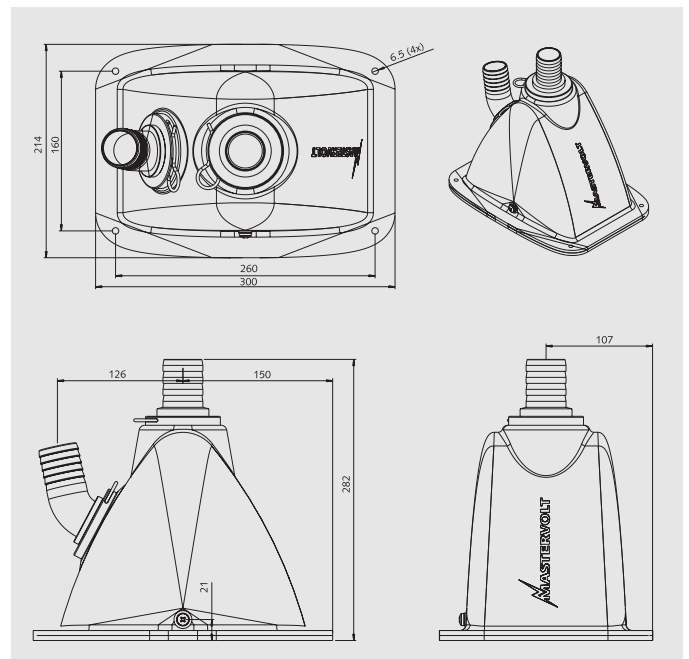
Dimensions in mm of the Delta silencer/waterlock.
